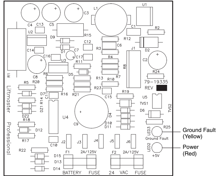
Figure 12 - Power Supply Board LED Descriptions
